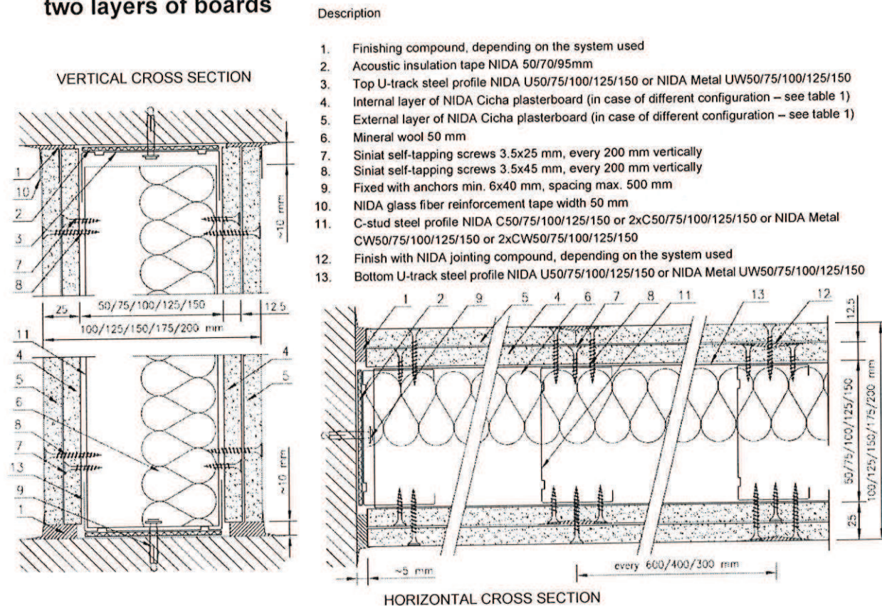
Fig. no. 1. Vertical and horizontal cross-section of anti-burglar non-loadbearing partition wall with a single framework and two layers of boards.
